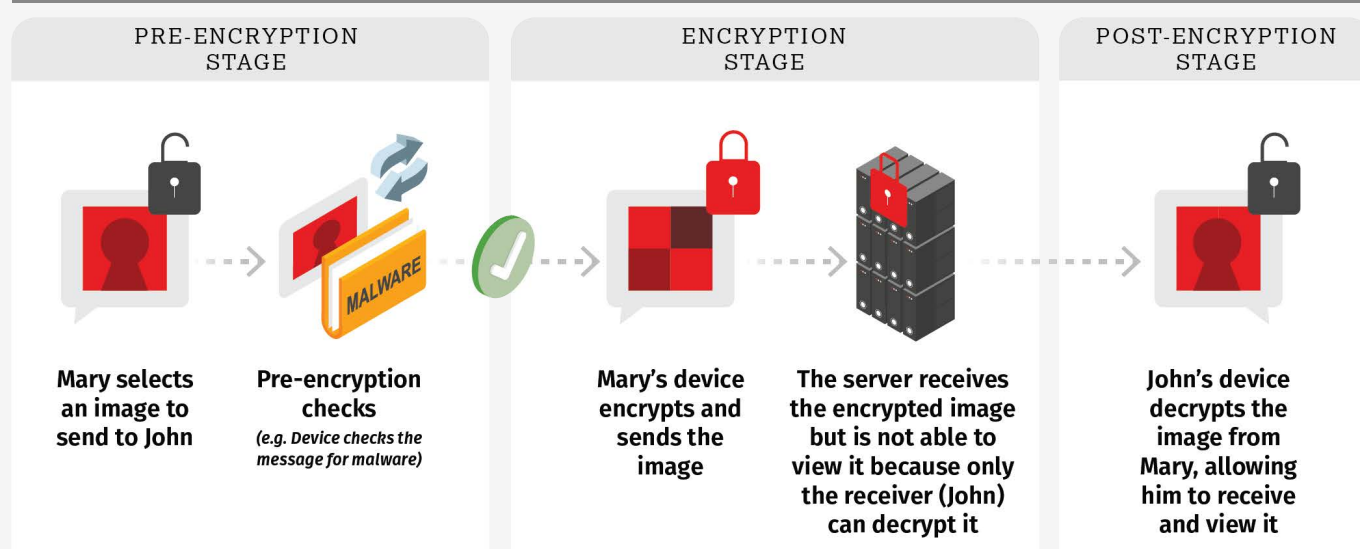
Figure 1: E2EE diagram
